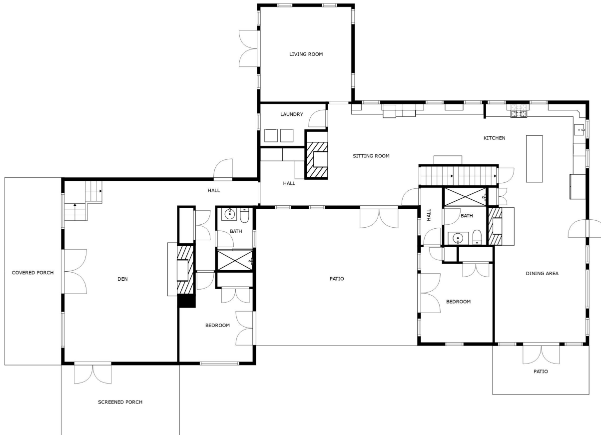
FLOOR 1
