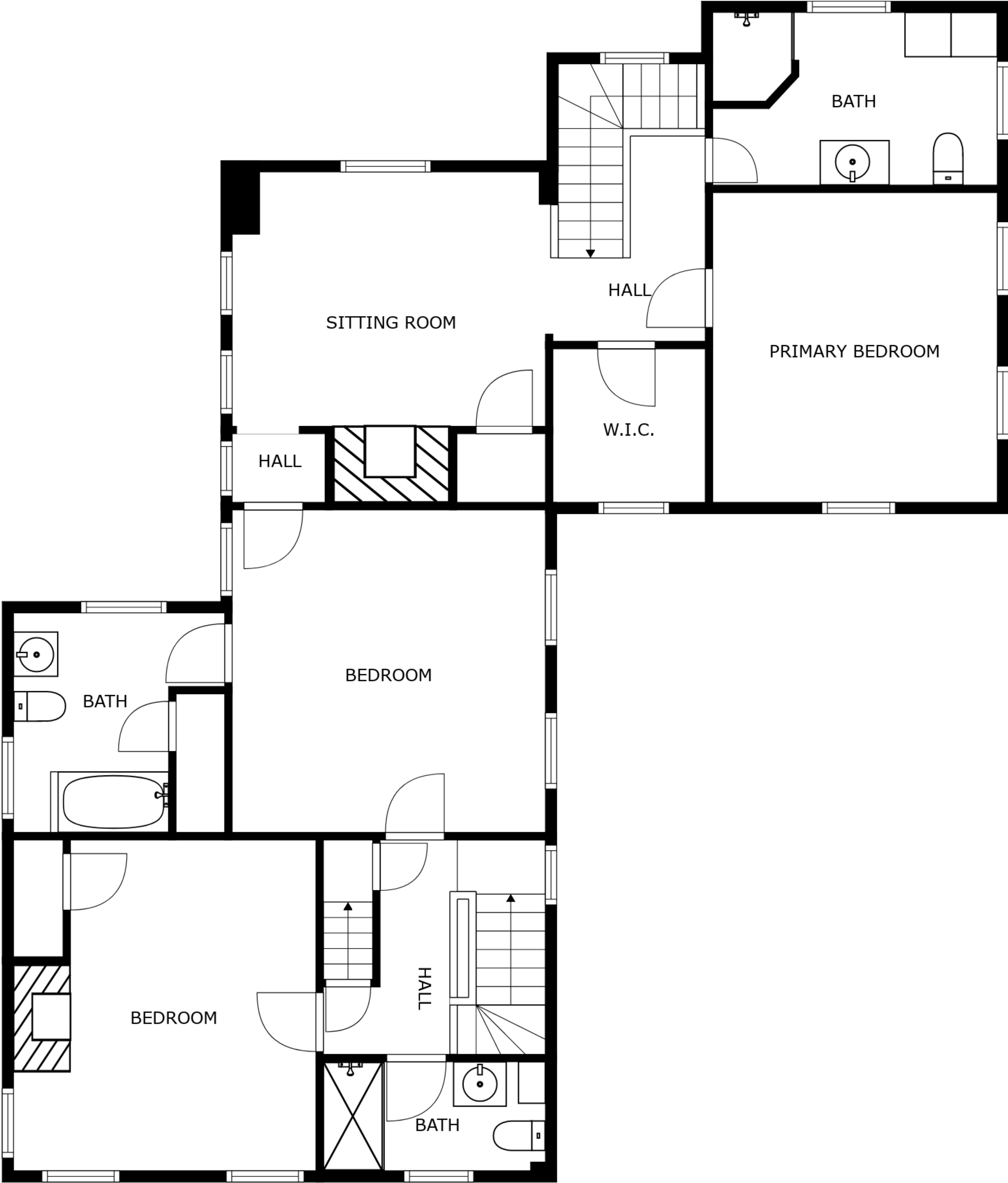
FLOOR 2
