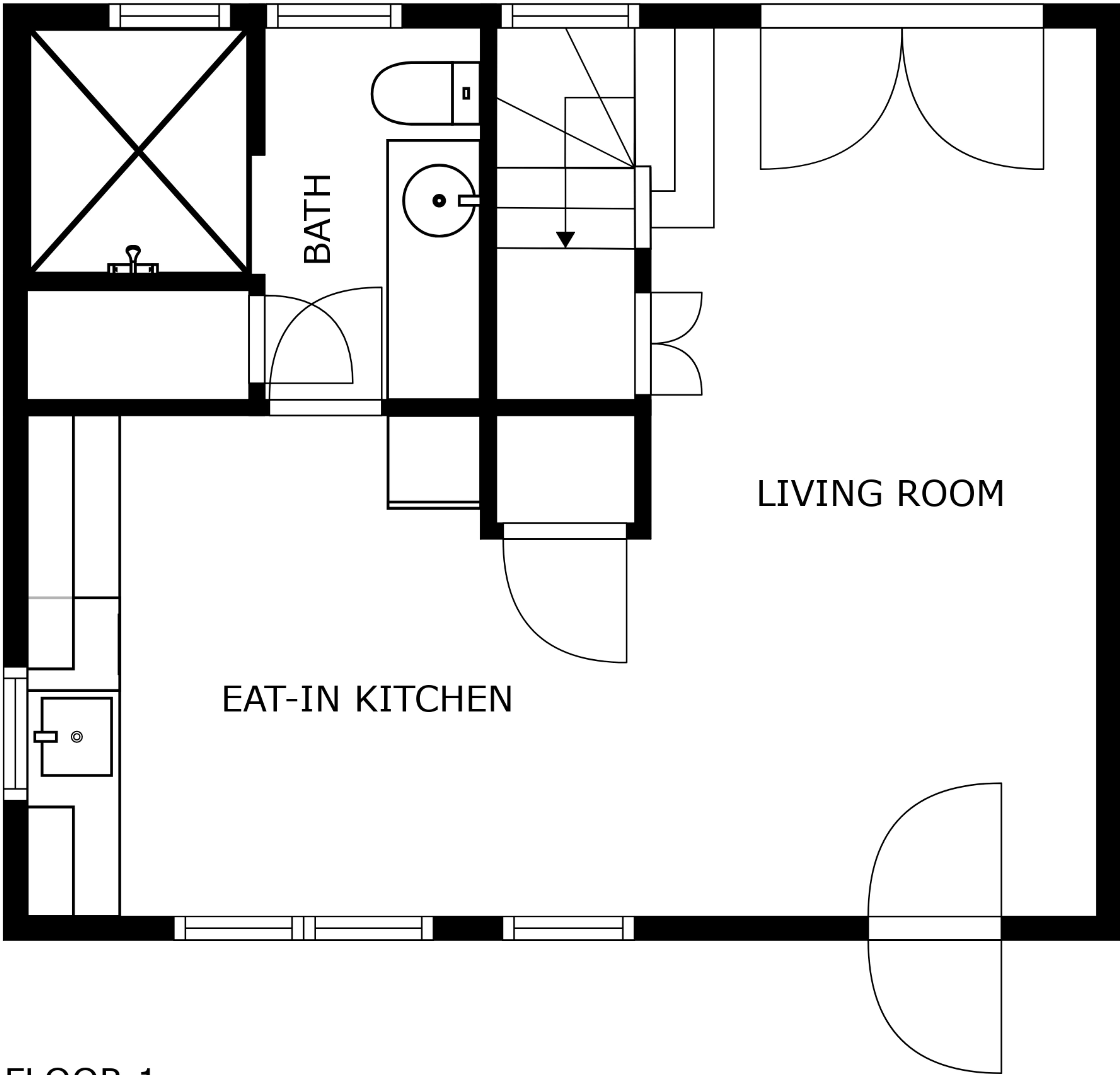
FLOOR 1
